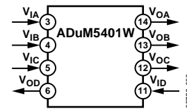
Figure 2. ADuM5401W
