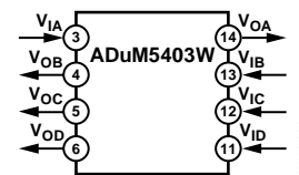
Figure 4. ADuM5403W
