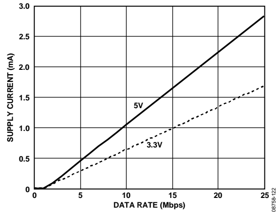
Figure 20. Typical I_{ISO(D)} Dynamic Supply Current per Output (15 pF Output Load)
